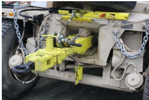
M989A1 TeleSwivel™ Lift Assist Kit (secured)
